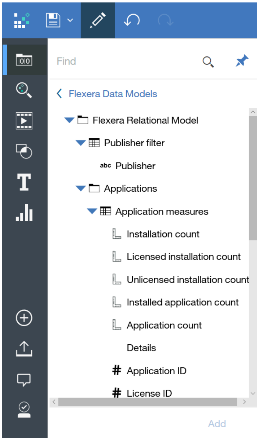
Figure 10: Relational model
